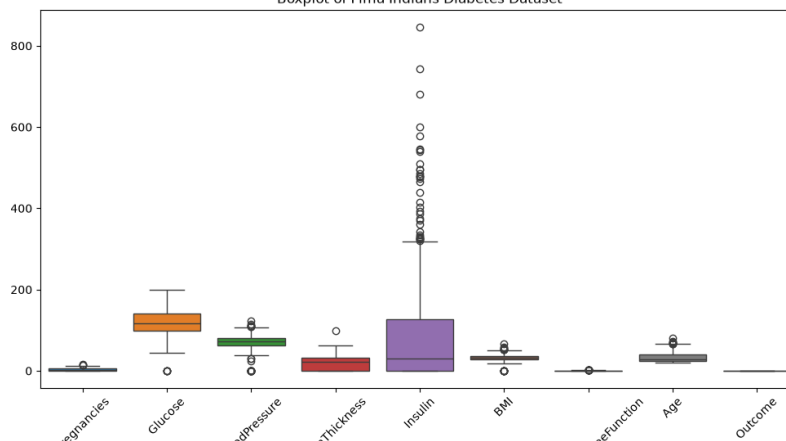
Boxplot of Pima Indians Diabetes Dataset
