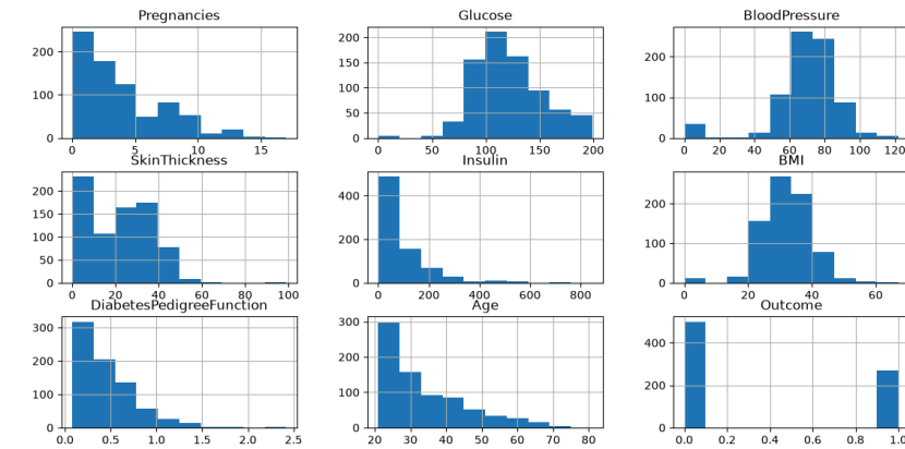
Histogram of Pima Indians Diabetes Dataset
