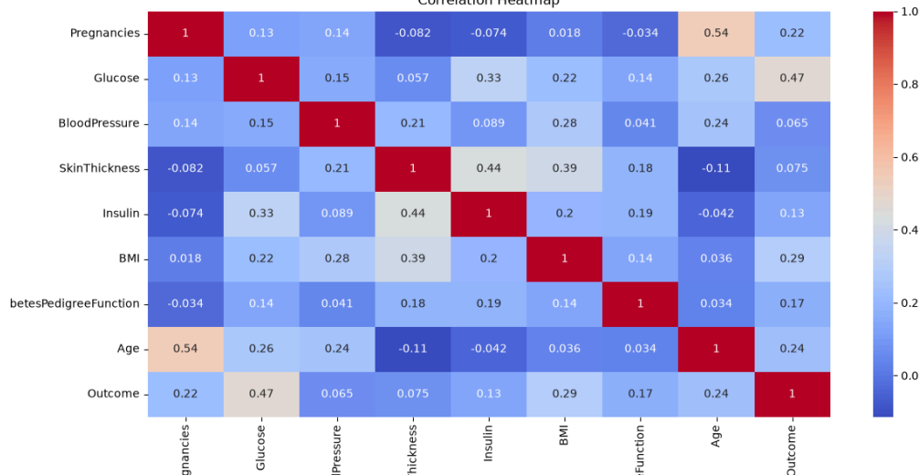
Correlation Heatmap
